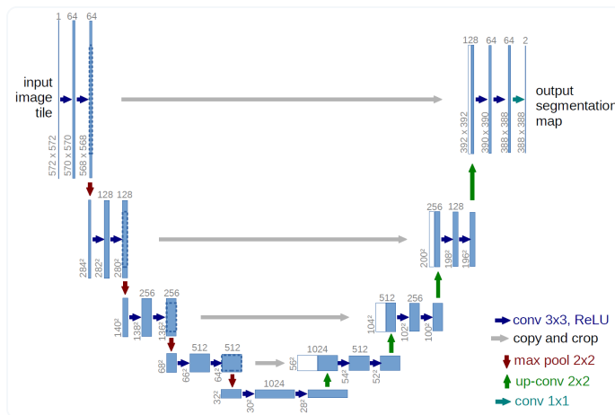
Architecture of U-Net ( source )
