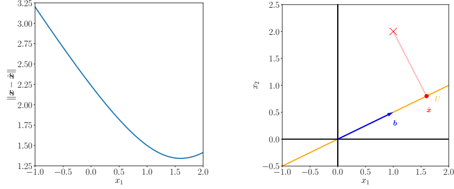
Figure 10.3 Optimal projection of a vector \mathbf{x} \in \mathbb{R}^2 onto a one-dimensional subspace (continuation from Figure 10.2). (a) Distances \|\mathbf{x} - \tilde{\mathbf{x}}\| for some \tilde{\mathbf{x}} \in U . (b) Orthogonal projection and optimal coordinates.
